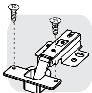
Bisagra parche/ Full overlay hinge
