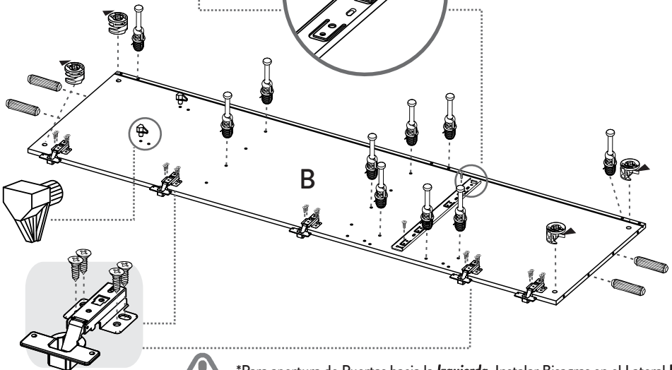
Bisagra parche/ Full overlay hinge
